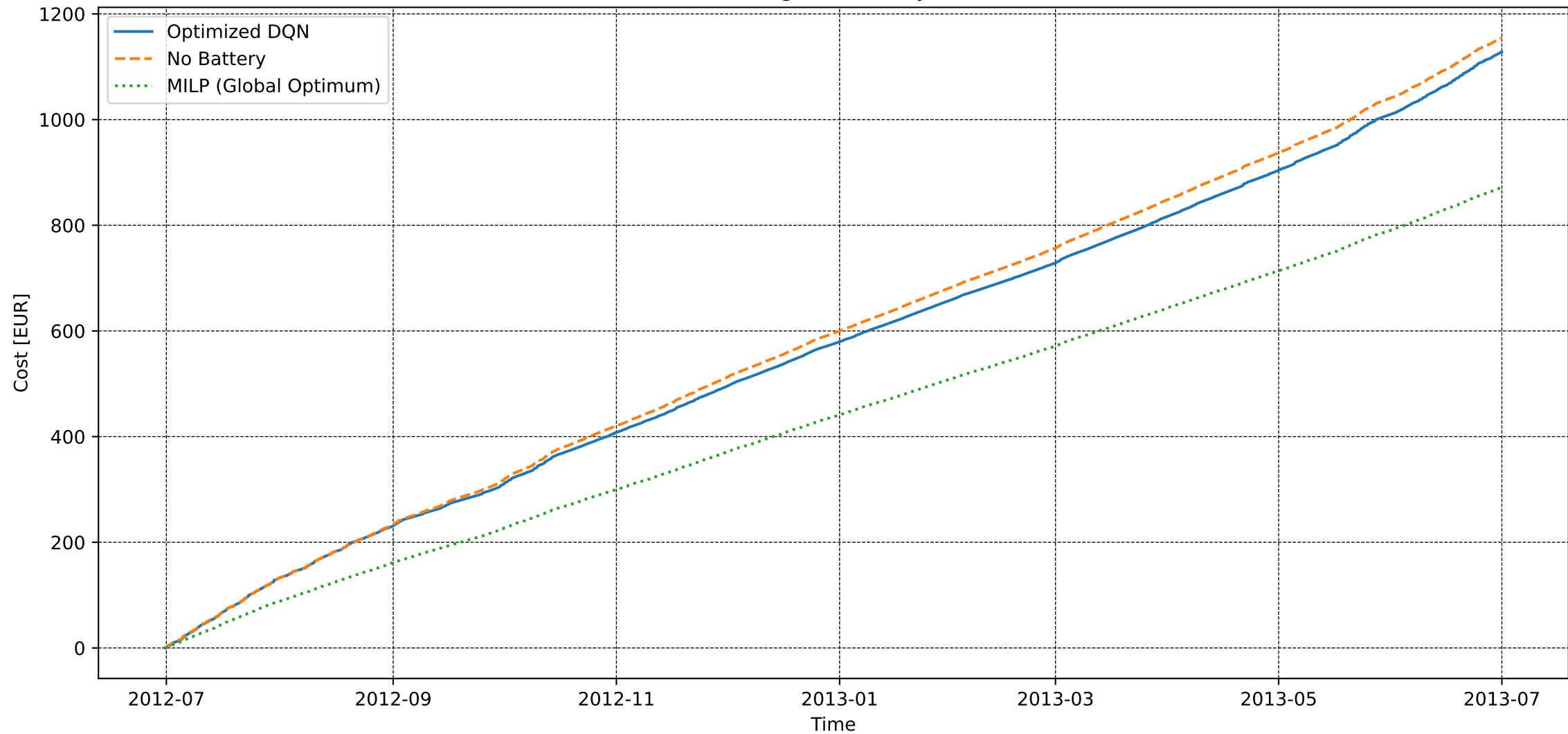
User 247 - Basic Training - Electricity Cost [DQN vs MILP]
